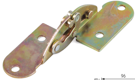
SAGRA 2 Bisagra para tapas de mesa 20/22mm. Folding table hinge for 20/22mm.
